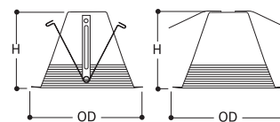
ERT713WHTTS ERT713WHT Height: OD: 5-3/8" [136mm] 7-1/4" [184mm]
