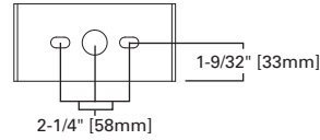
TRUNNION DETAIL
