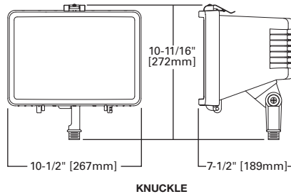
KNUCKLE
