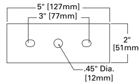
TRUNNION DETAIL
