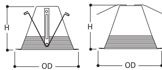
ERT713TS ERT713 Height: OD: 5" [127mm] 7-1/4" [184mm]
