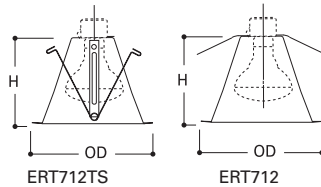
ERT712TS ERT712 Height: OD: 5-3/8" [136mm] 7-1/4" [184mm]
