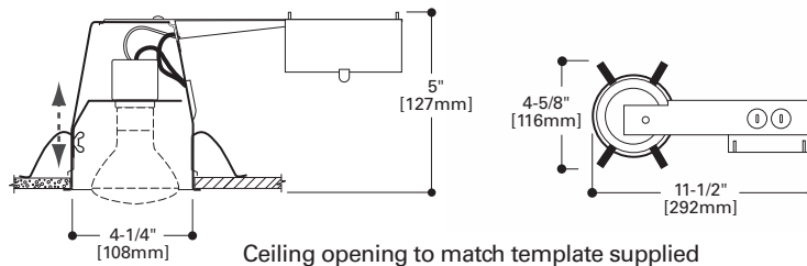
Ceiling opening to match template supplied
